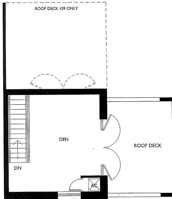
LEVEL THREE
