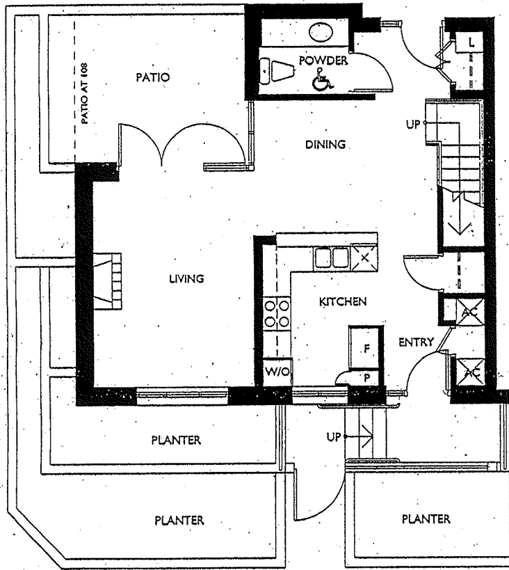
LEVEL ONE
