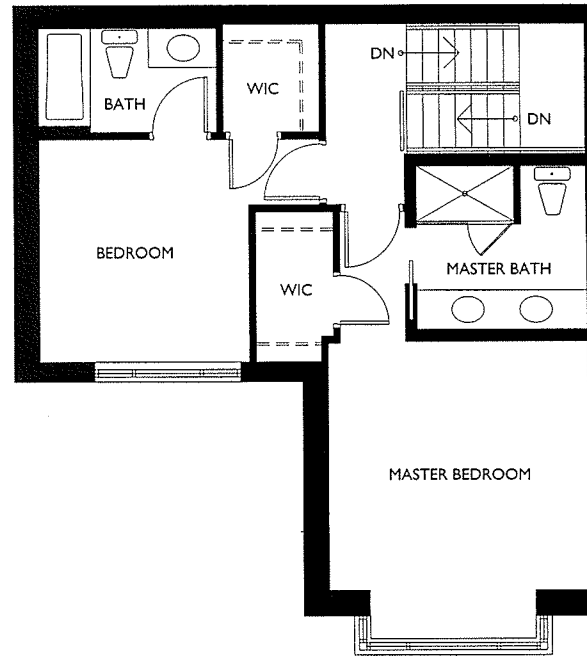
LEVEL TWO
