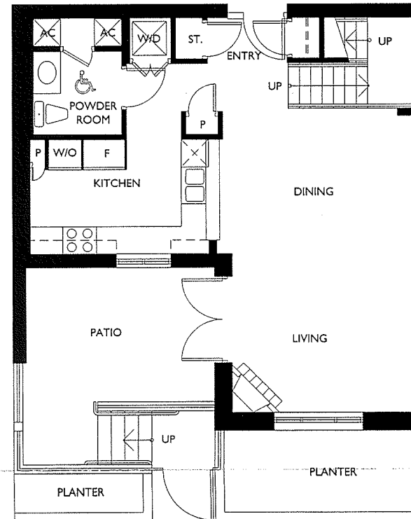
LEVEL ONE
