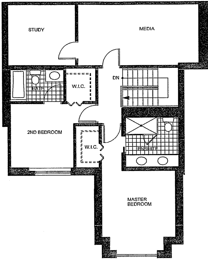
LAYOUT FOR UPPER FLOOR SHOWN, 1079 SQ. FT.
