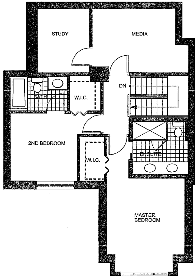
LAYOUT FOR UPPER FLOOR SHOWN, 976 SQ. FT.
