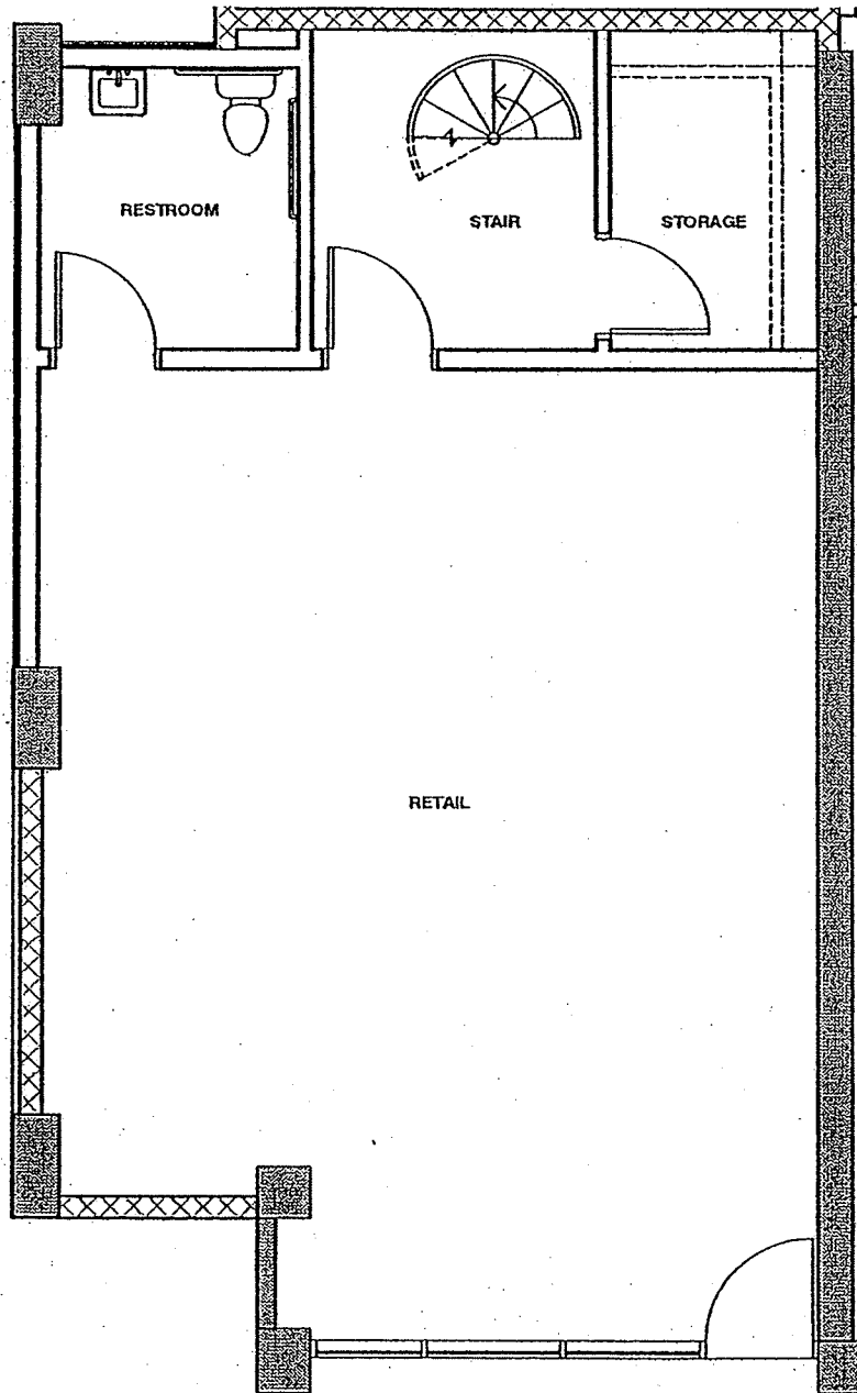
UNIT C - FIRST FLOOR
