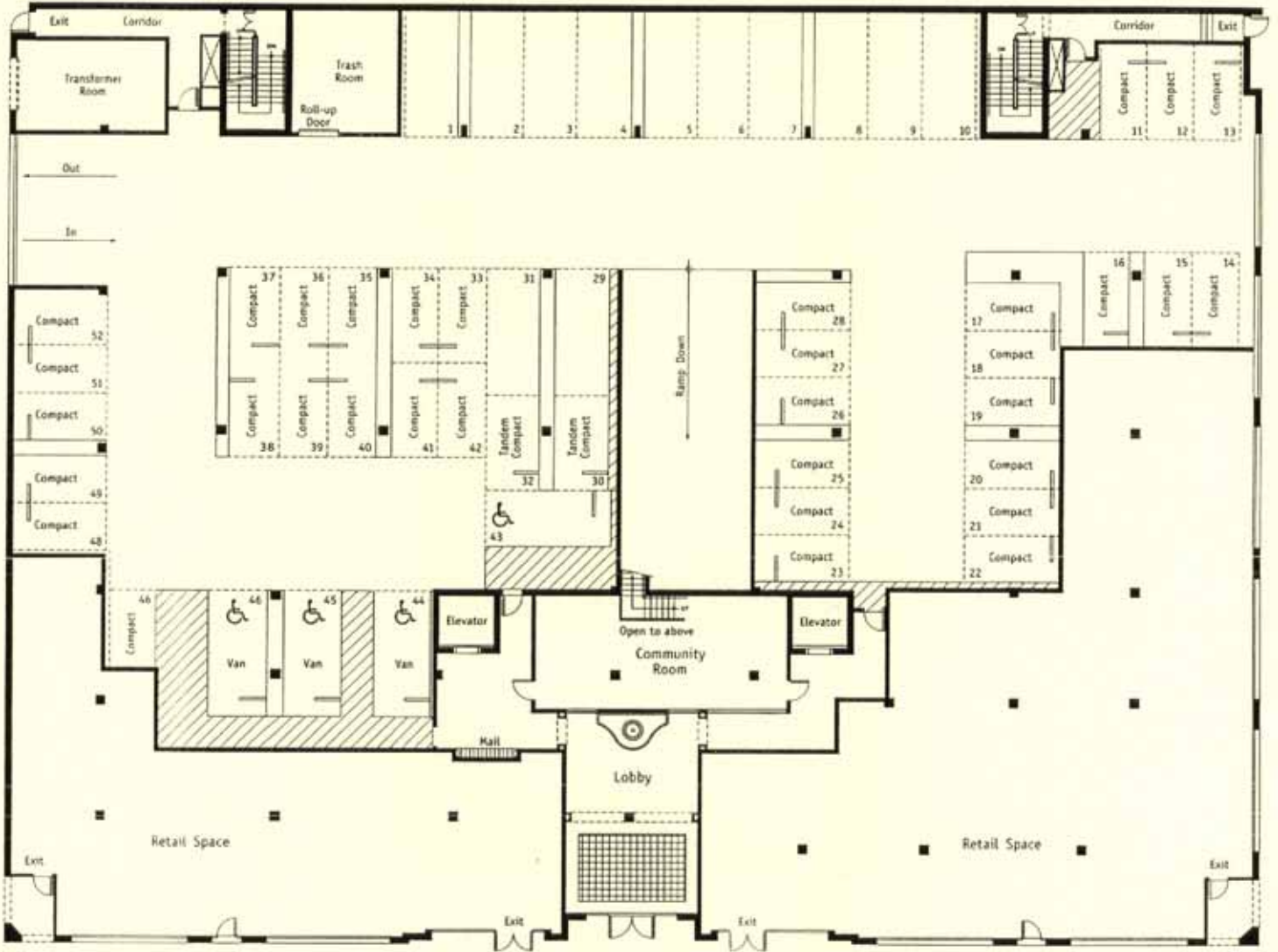
Level 1 & Parking
